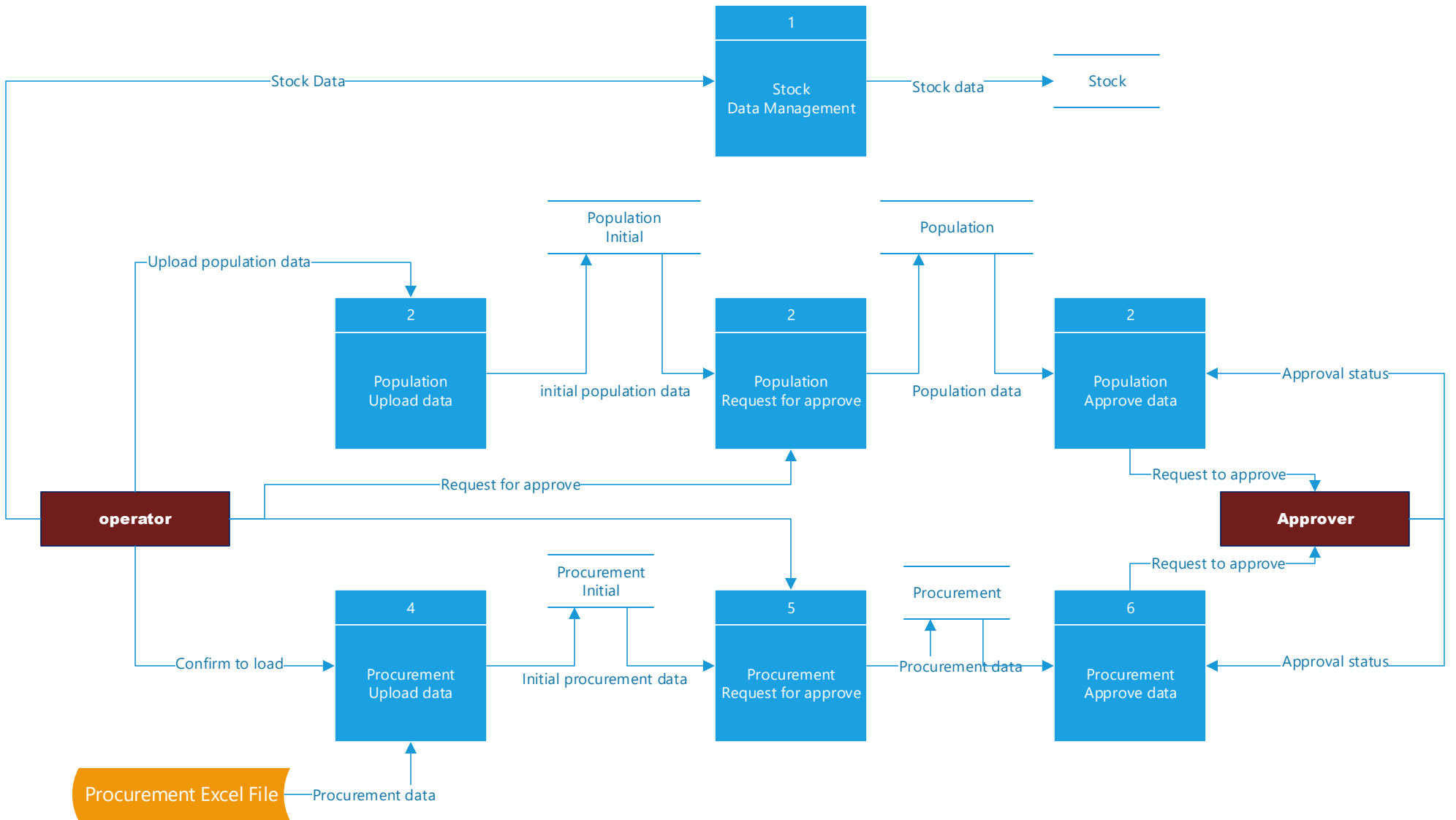
DFD: Level 2:Vaccine Management
