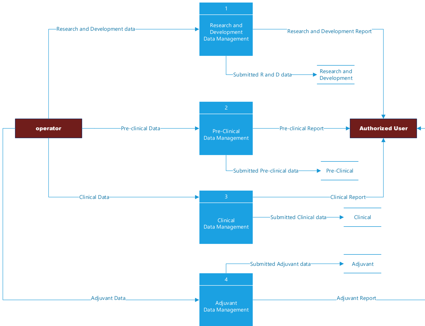
DFD: Level 2: Research And Development
