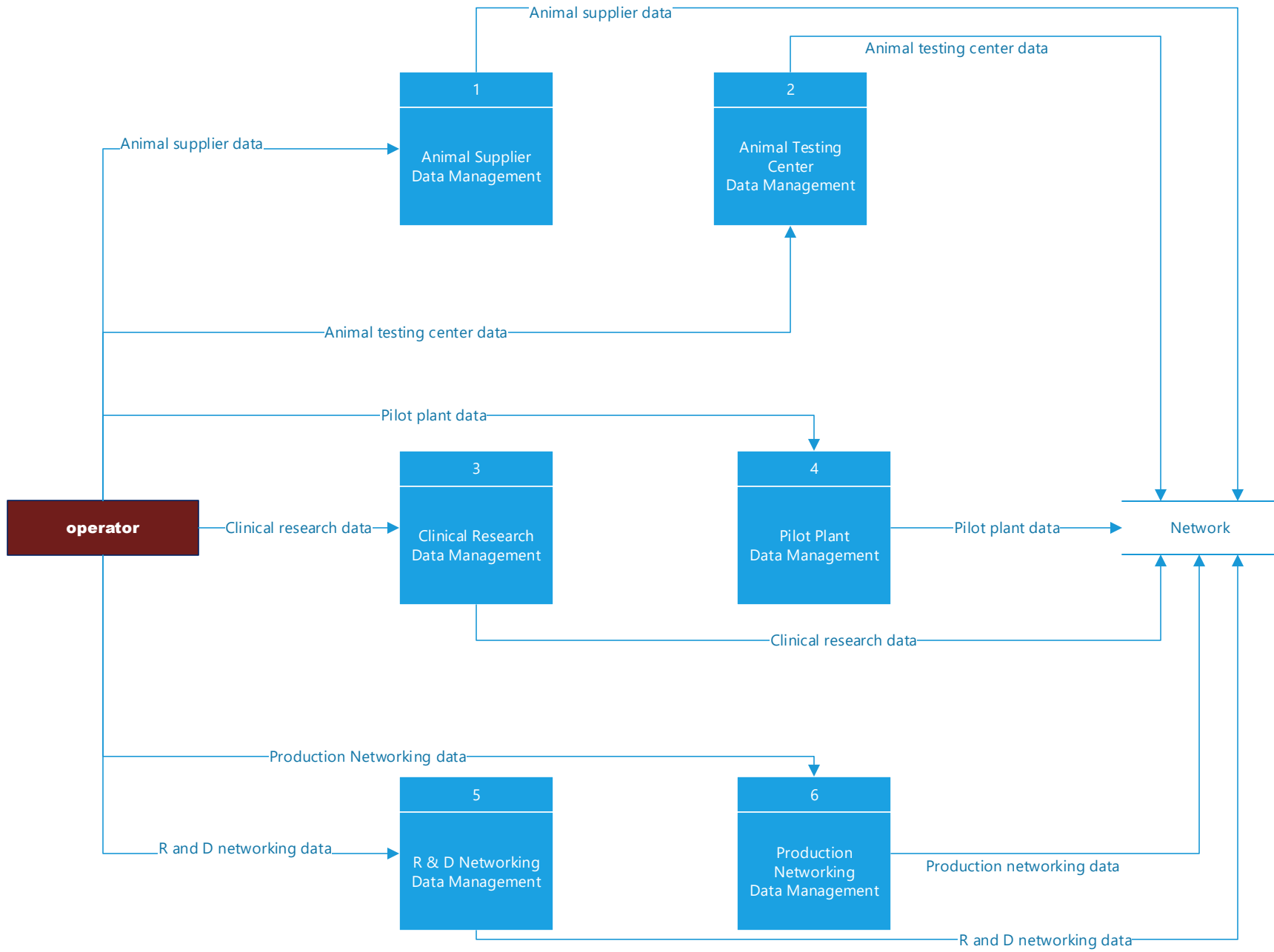
DFD: Level 2: Infrastructure and Networking
